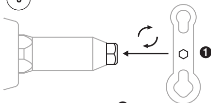
Use the special wrench 1 to screw the nosepiece.
